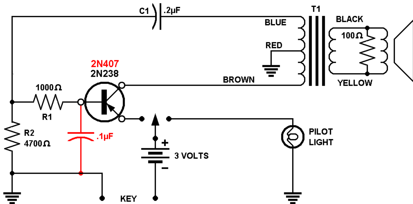
Heathkit CO-1 Schematic 1964 changes shown in red
