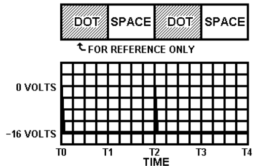
TRIGGER PULSE AT JUNCTION OF C51 AND D50 WITH KEY LEVER IN DOT POSITION
