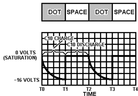
Q1 COLLECTOR VOLTAGE Figure 11
