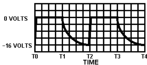
Q2 COLLECTOR VOLTAGE
