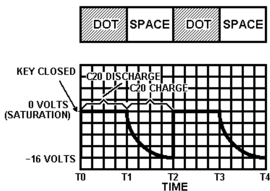
Q2 COLLECTOR VOLTAGE Figure 10
