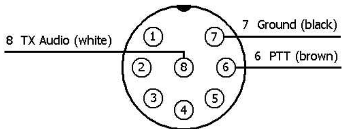
Female Connector (Wiring Side)
