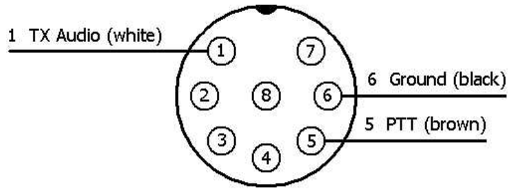
Female Connector (Wiring Side)
