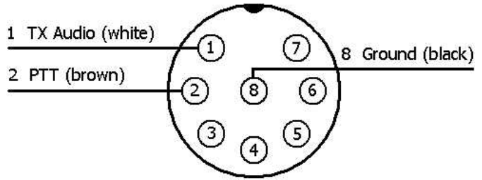
Female Connector (Wiring Side)
